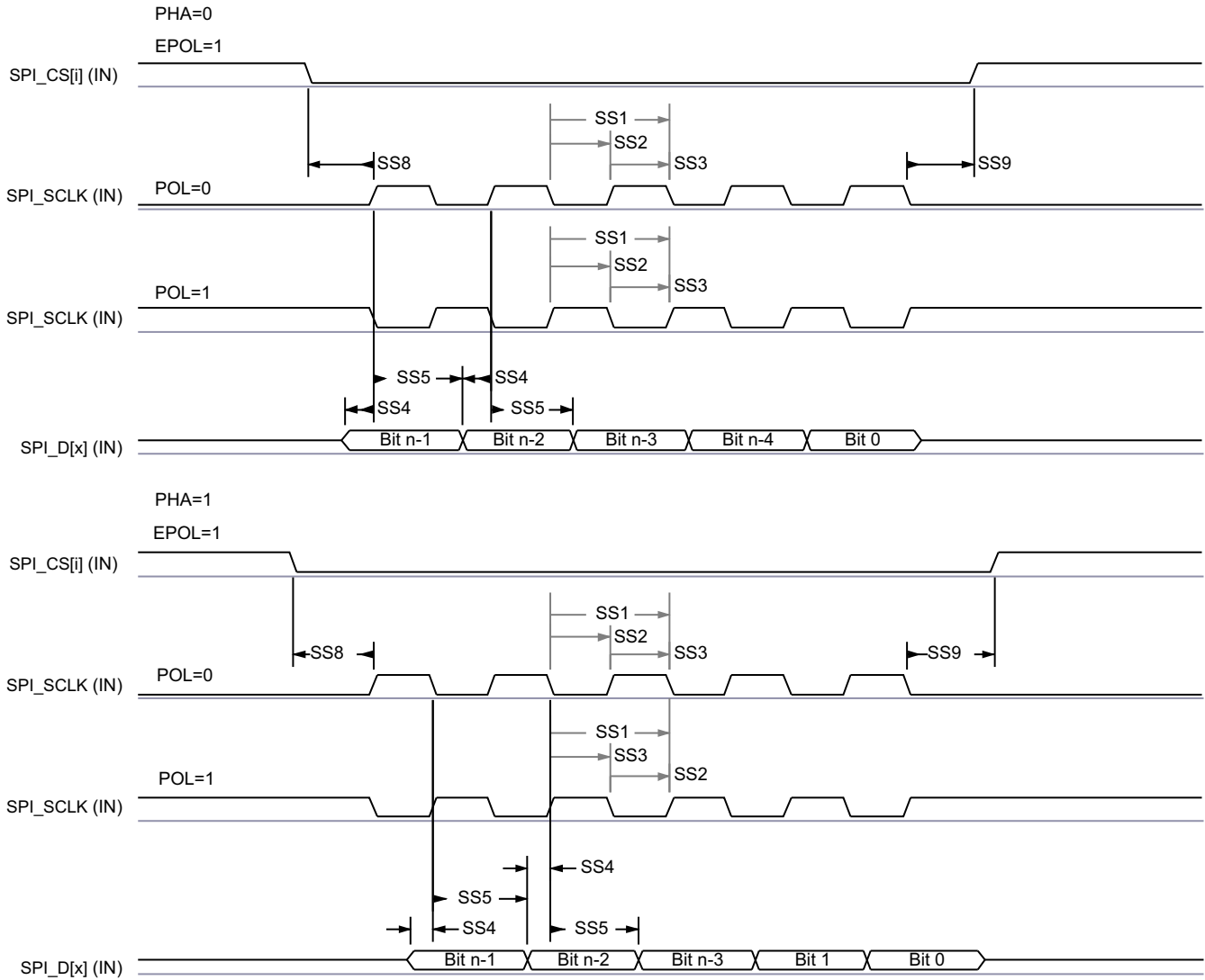
图 7-36. SPI Slave Mode Receive Timing
