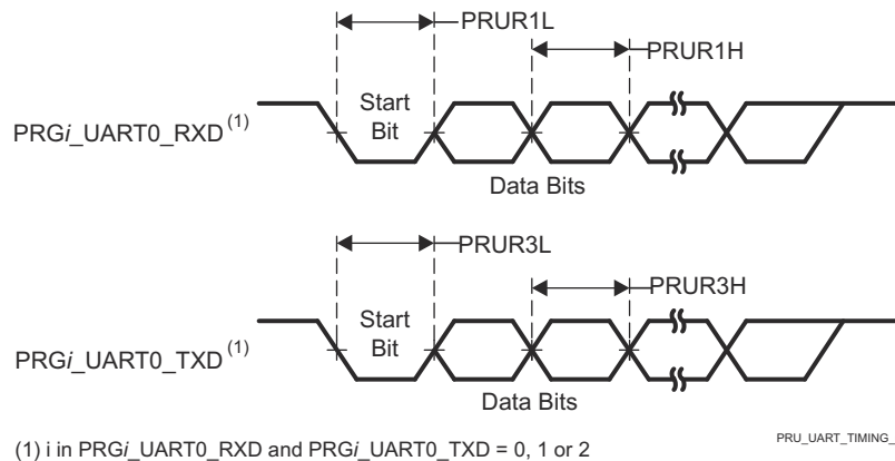
图 7-57. PRU_ICSSM UART Timing Requirements and Switching Characteristics
