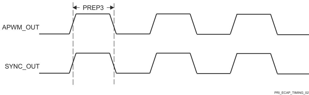
图 7-59. PRU_ICSSM ECAP Switching Characteristics
