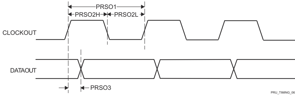
图 7-48. PRU_ICSSM PRU Shift Out Timing
