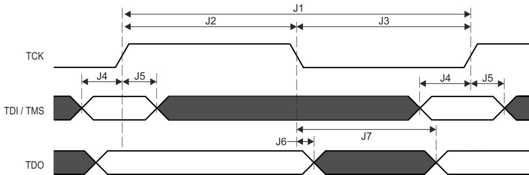
图 7-62. JTAG Timing Requirements and Switching Characteristics
