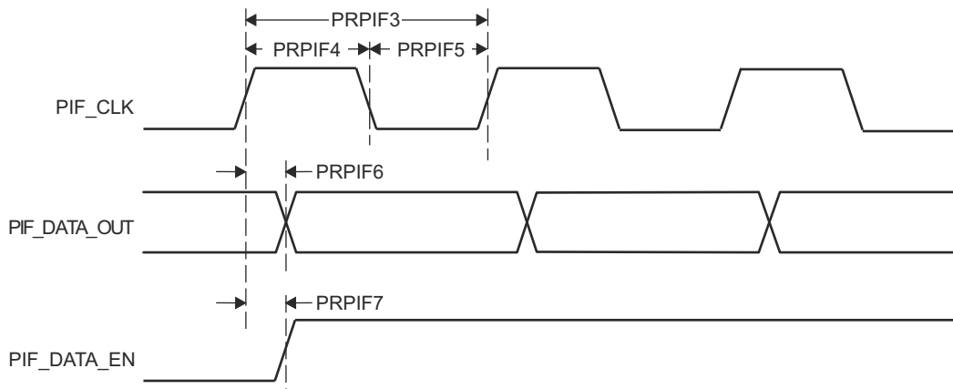
图 7-52. PRU_ICSSM PRU Peripheral Interface Switching Characteristics
