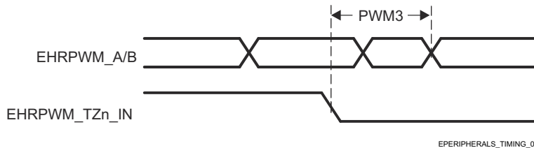
图 7-12. EHRPWM_TZn_IN to EHRPWM_A/B Forced Switching Characteristics
