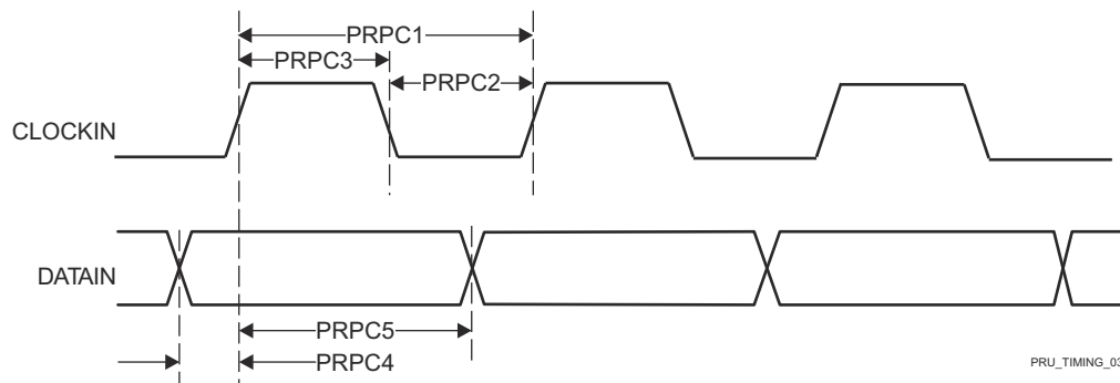
图 7-45. PRU_ICSSM PRU Parallel Capture Timing Requirements - Rising Edge Mode
