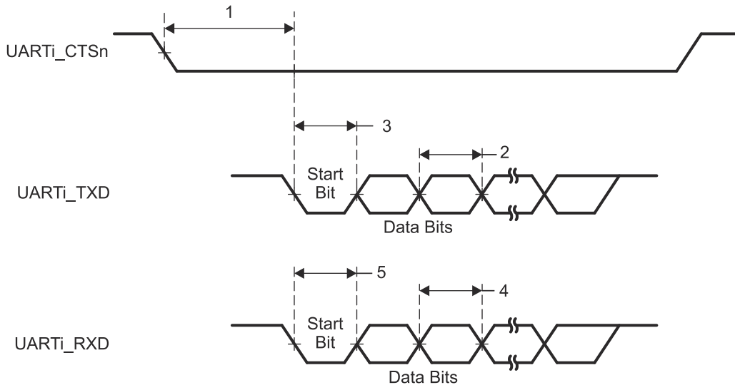
图 7-60. UART Timing Requirements and Switching Characteristics
