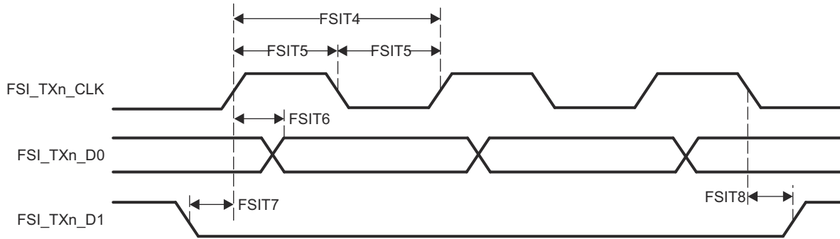
图 7-17. FSI Switching Characteristics - SPI Mode
