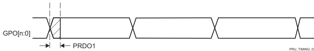
图 7-44. PRU_ICSSM PRU Direct Output Timing
