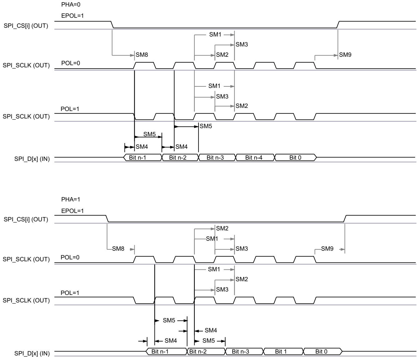
图 7-34. SPI Master Mode Receive Timing
