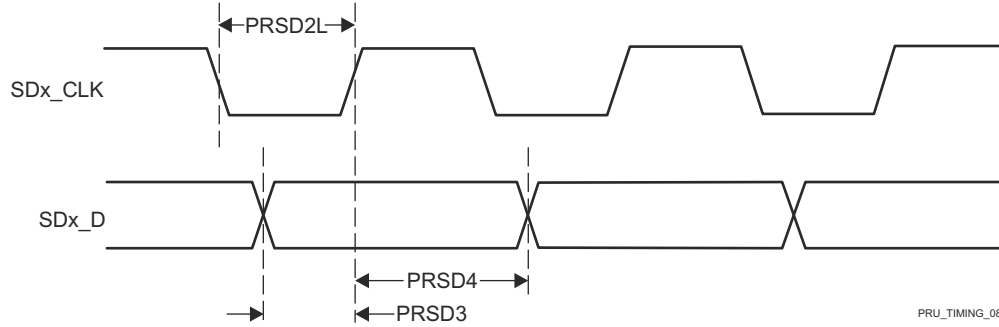
图 7-50. PRU_ICSSM PRU SD_CLK Rising Active Edge
