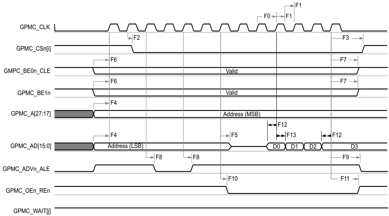
图 7-20. GPMC and NOR Flash—Synchronous Burst Write (GPMCFCLKDIVIDER = 0)
