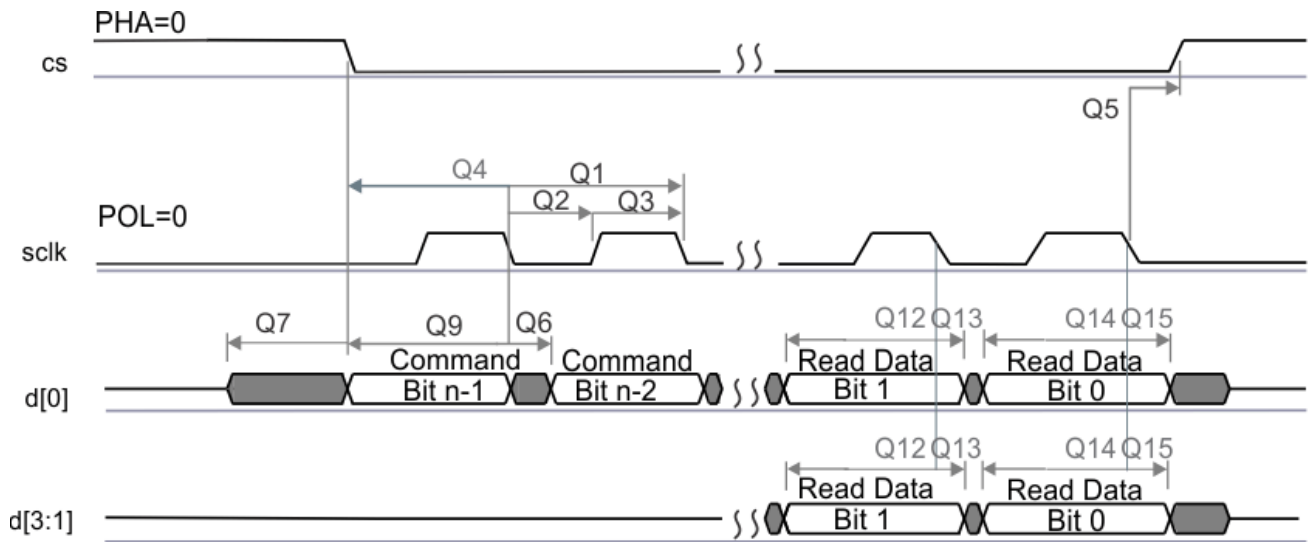
图 7-42. QSPI Timing Requirements
