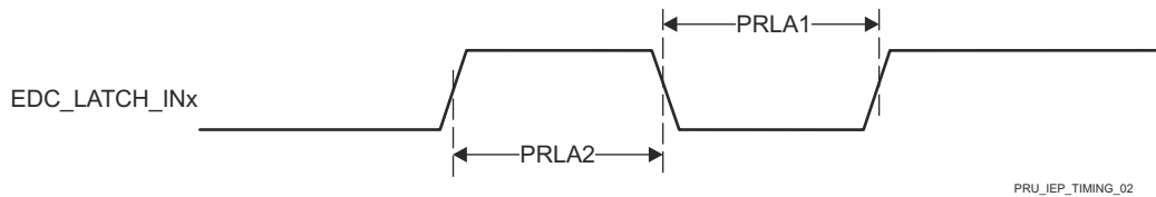
图 7-56. PRU_ICSSM IEP LATCH_INx Timing Requirements
