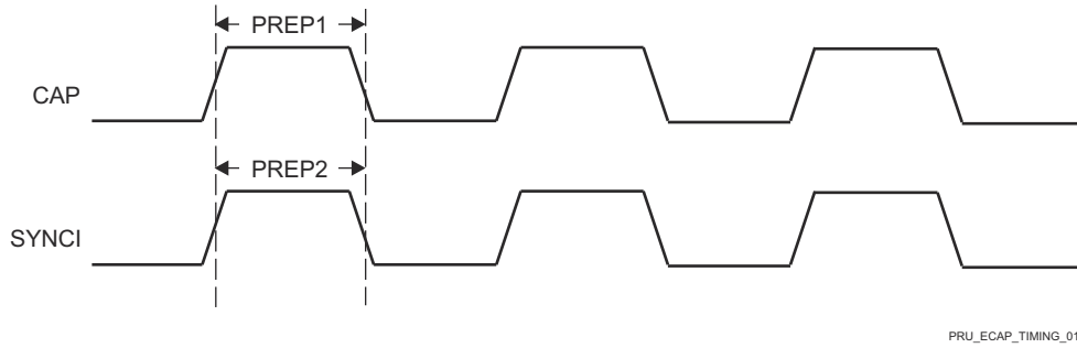
图 7-58. PRU_ICSSM ECAP Timing
