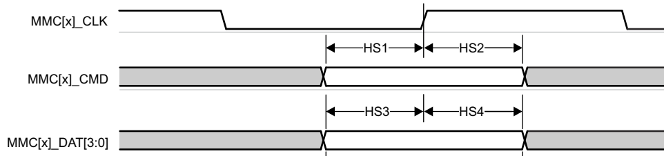
图 7-40. MMC1 - High Speed - Receive Mode
