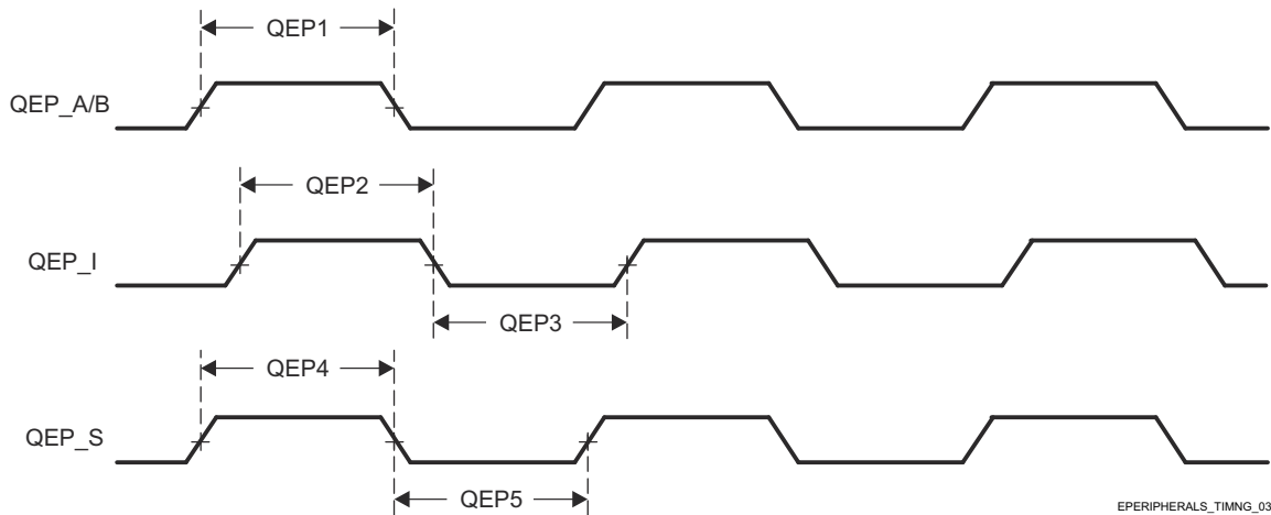
图 7-14. EQEP Timing Requirements
