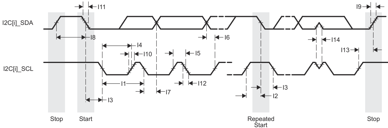
图 7-33. I2C Receive Timing
