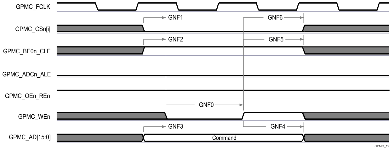
图 7-29. GPMC and NAND Flash — Command Latch Cycle
