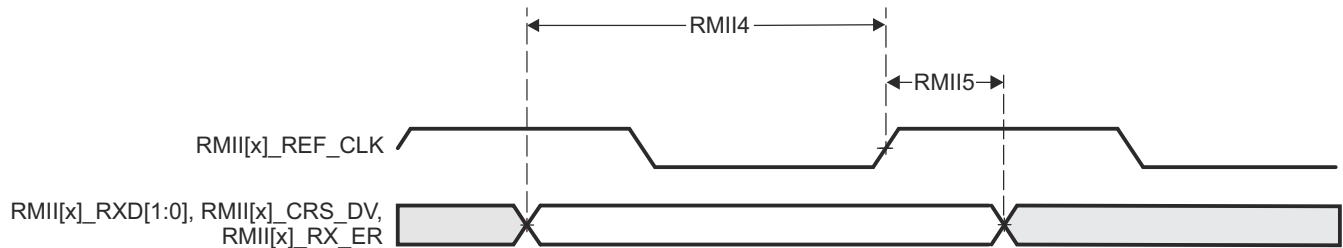
图 7-4. CPSW3G RMII[x]_RXD[1:0], RMII[x]_CRS_DV, RMII[x]_RX_ER Timing Requirements - RMII Mode
