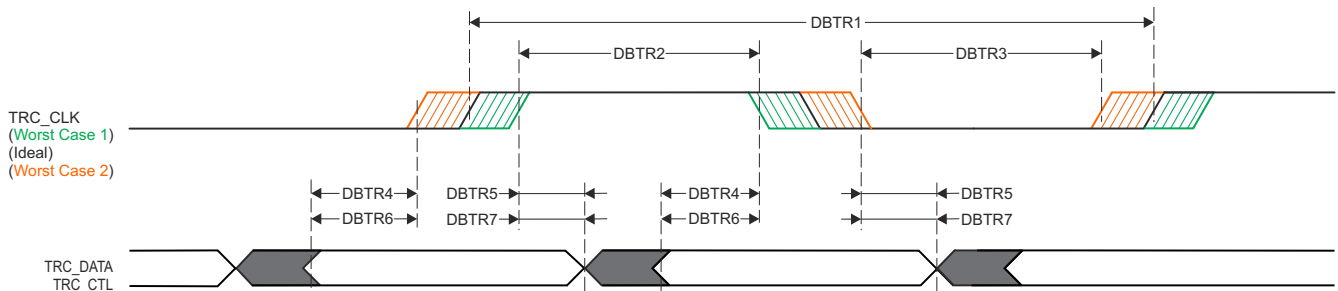
图 7-61. Trace Switching Characteristics
