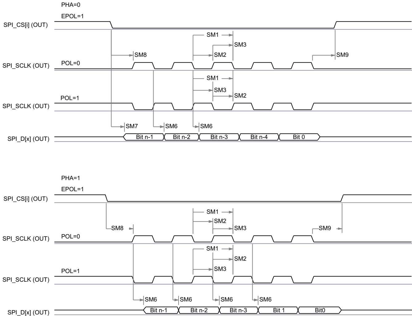
图 7-35. SPI Master Mode Transmit Timing
