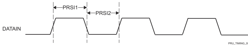
图 7-47. PRU_ICSSM PRU Shift In Timing
