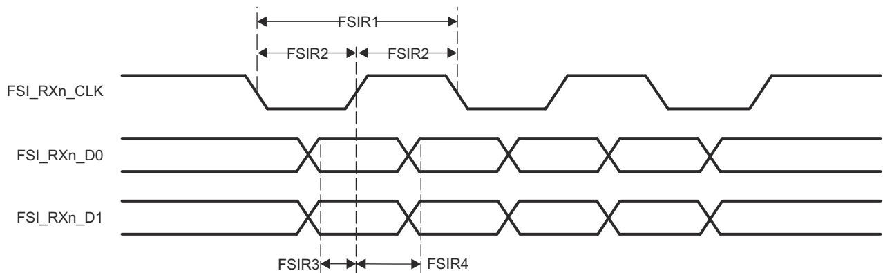
图 7-15. FSI Timing Requirements
