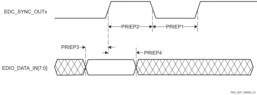
图 7-54. PRU_ICSSM IEP SYNC Timing Requirements
