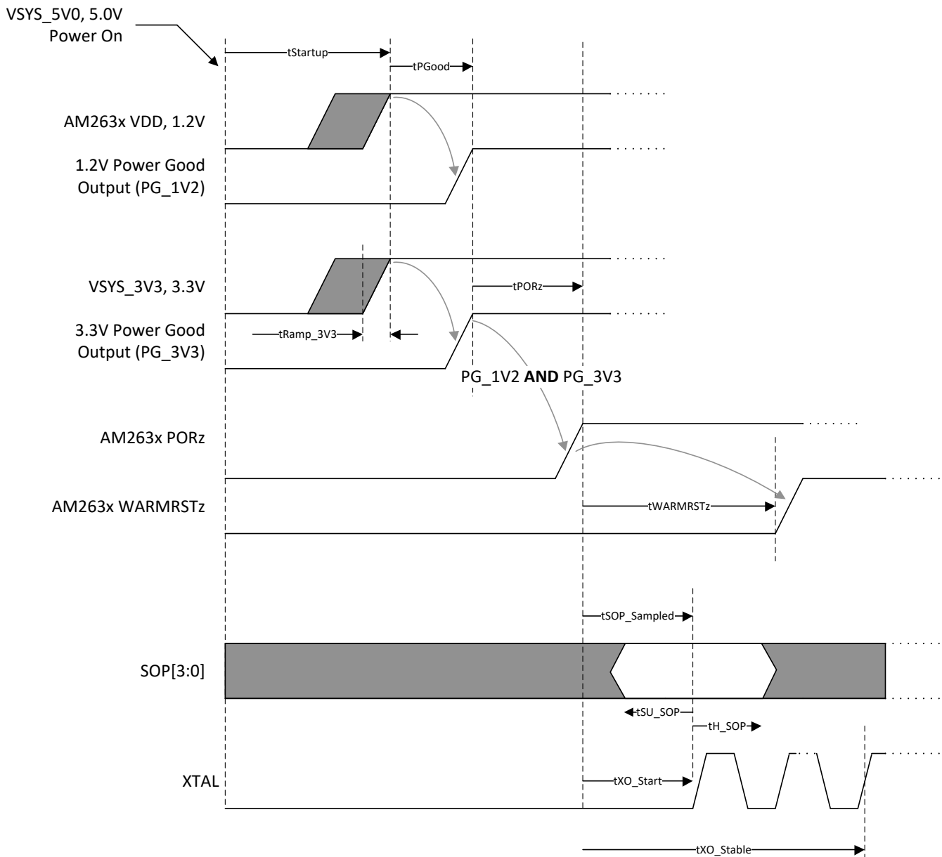
图 7-1. Power-Up Sequencing
