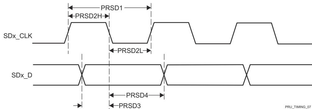
图 7-49. PRU_ICSSM PRU SD_CLK Falling Active Edge
