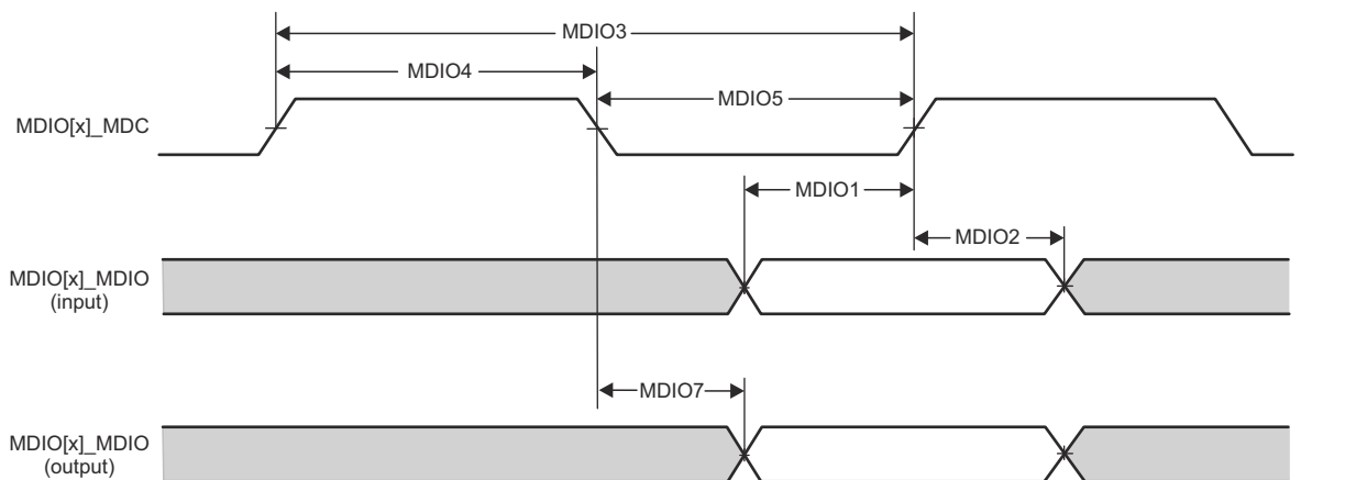
图 7-2. CPSW3G MDIO Timing Requirements and Switching Characteristics
