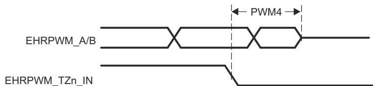
图 7-13. EHRPWM_TZn_IN to EHRPWM_A/B Hi-Z Switching Characteristics
