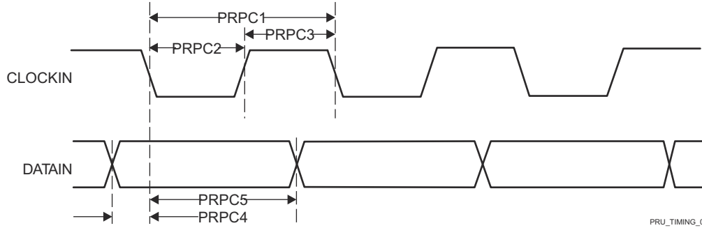
图 7-46. PRU_ICSSM PRU Parallel Capture Timing Requirements - Falling Edge Mode
