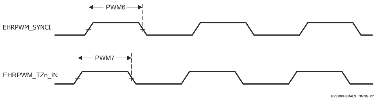
图 7-10. EPWM Timing Requirements
