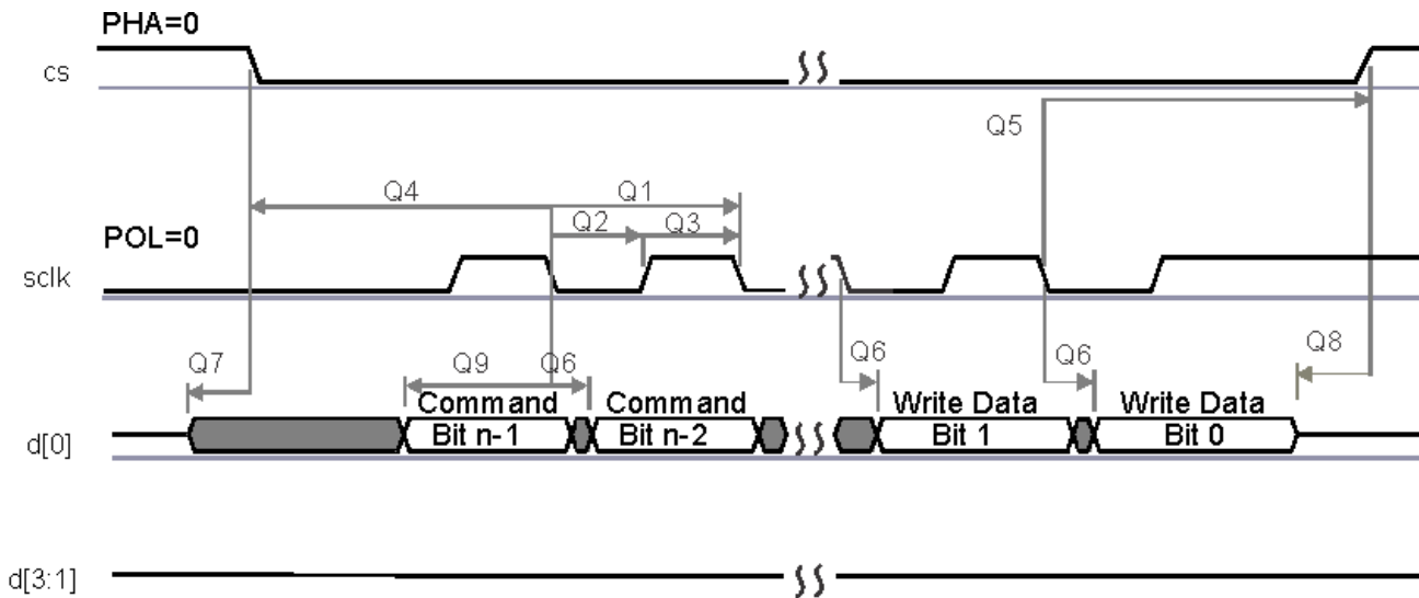
图 7-43. QSPI Switching Characteristics
