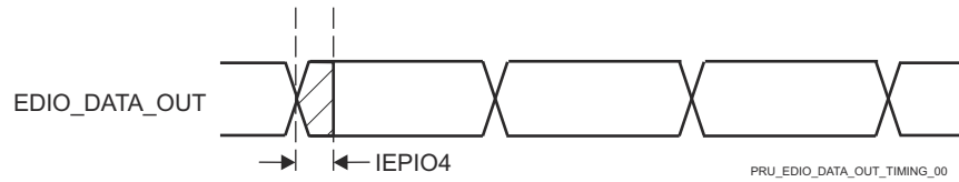
图 7-55. PRU_ICSSM IEP Digital IOs Timing Requirements
