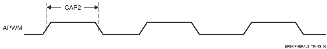
图 7-9. ECAP Switching Characteristics
