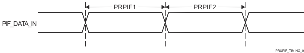
图 7-51. PRU_ICSSM PRU Peripheral Interface Timing Requirements
